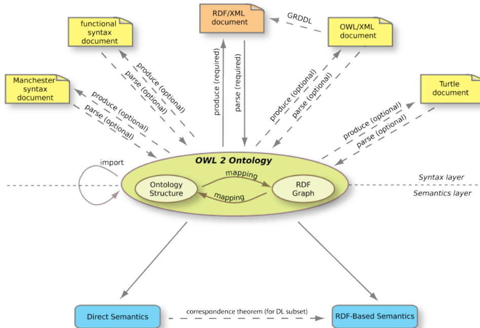
Figure 1. The Structure of OWL 2
